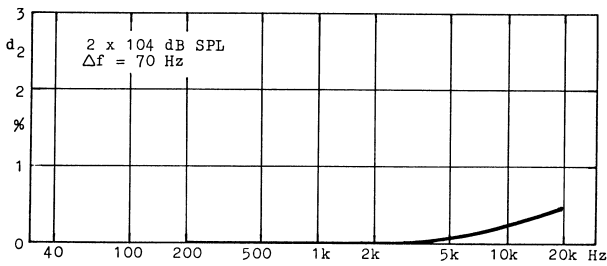
Fig.4: Correlation of frequency and intermodulation distortion (push-pull transducer)
