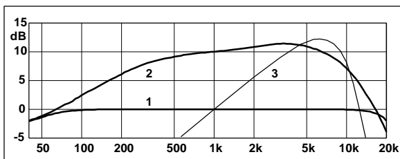
Fig.7: Damping
